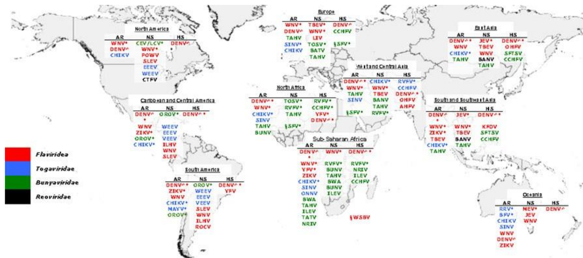
Figure: Overlapping distribution of selected arboviruses (Cleaton et al , PLoS Negl Trop Dis)
