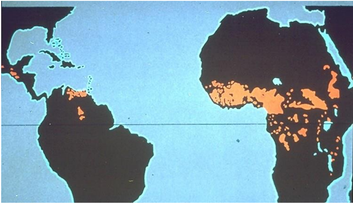
Map of endemic onchocerciasis areas.
